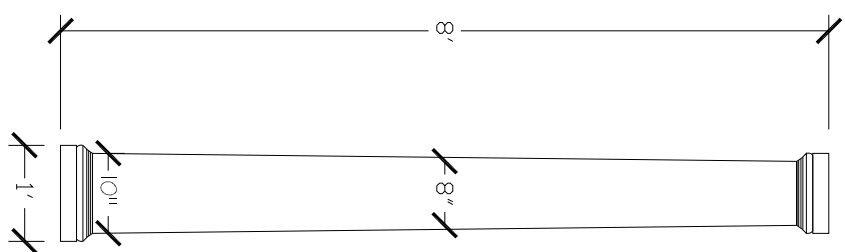
COLUMN 8 11 TAPERING TO 10 11 WIDE 8' TALL
