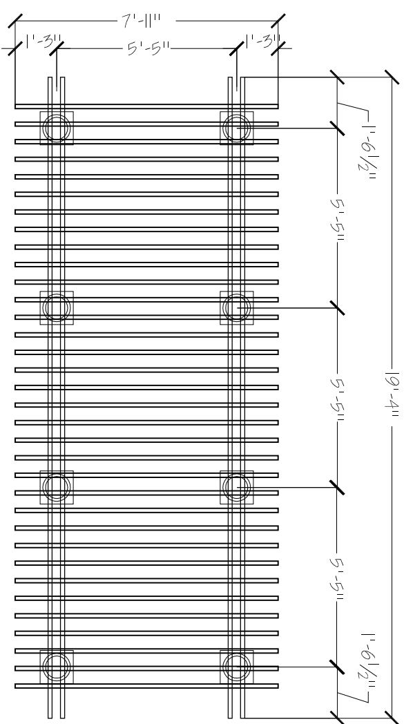
8 COLUMN
